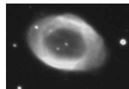
M57 – Ring Nebula
